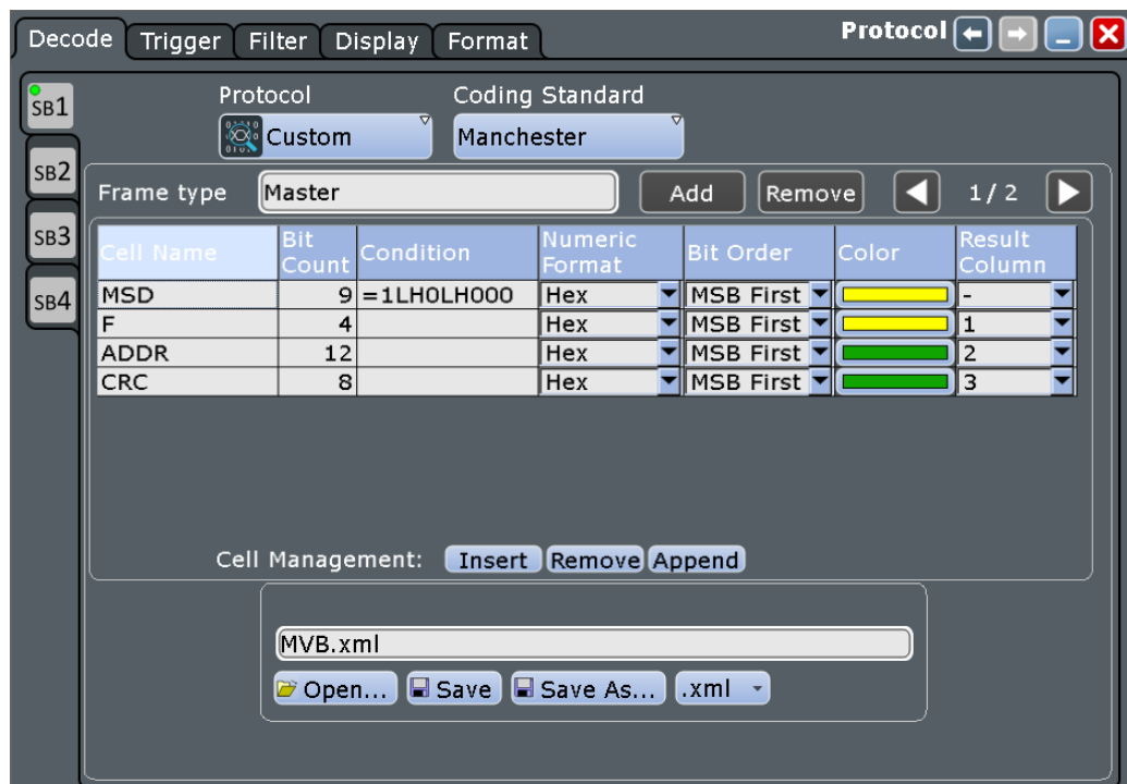
Figure 12-81: Example of a custom "MVB" frame format description (frame 1 of 2)
