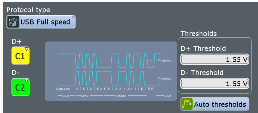
Figure 12-102: USB full speed protocol configuration
