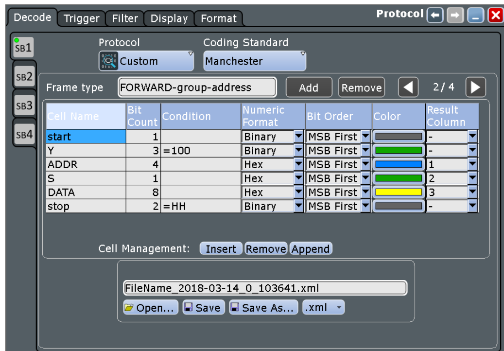
Figure 12-80: Example of a custom "DALI" frame format description (frame 2 of 4)
