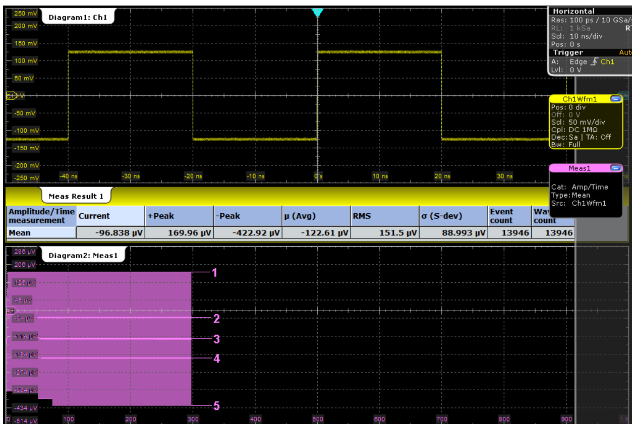
Figure 7-9: Long-term measurement with statistics
