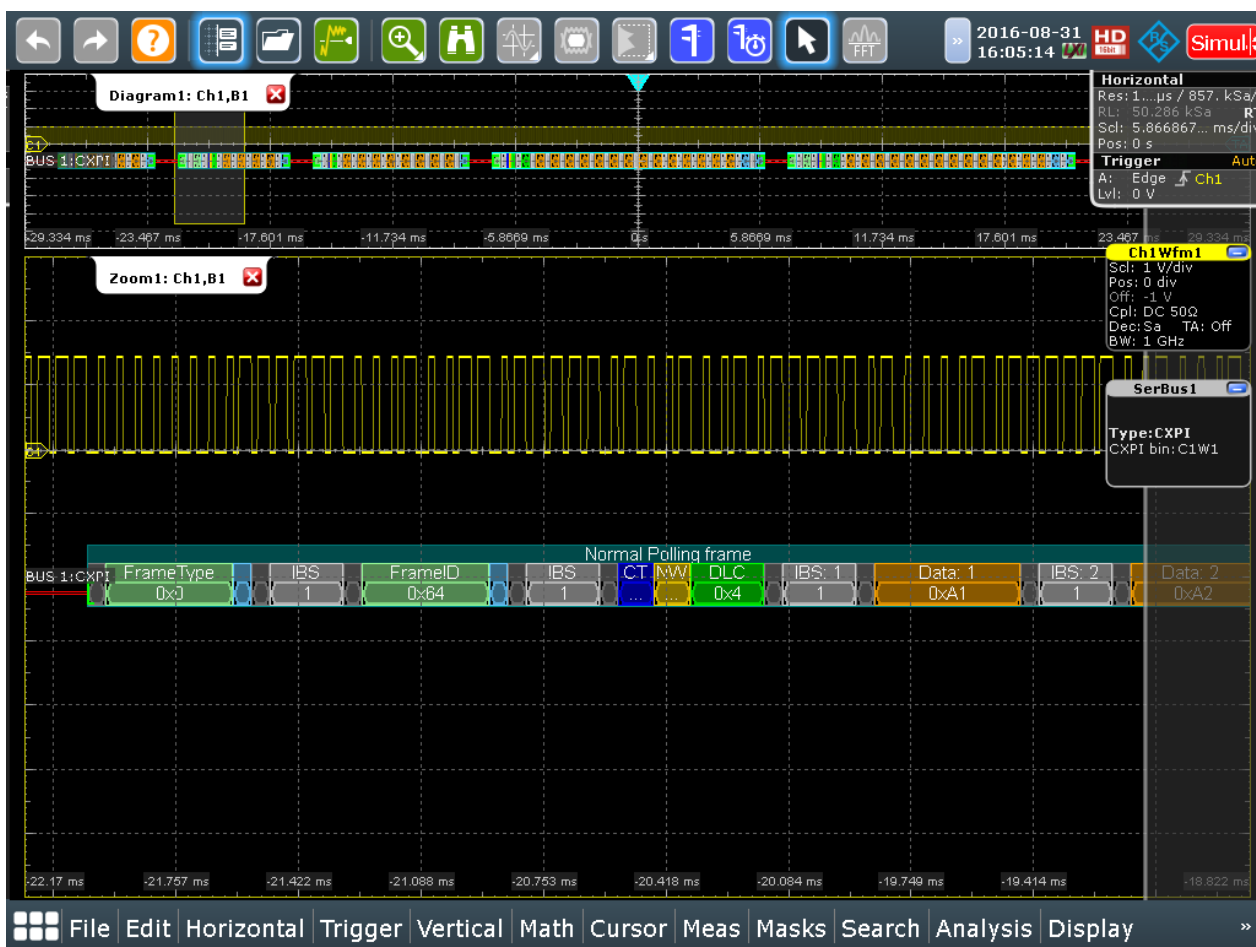
Figure 12-120: Decoded CXPI signal, normal polling frame
