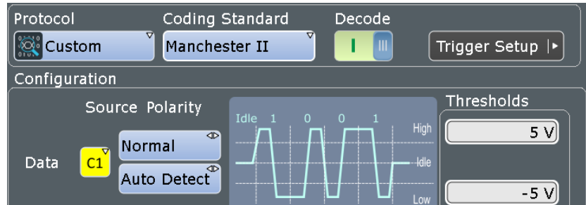
Figure 12-77: Custom serial bus coding configuration Manchester II
