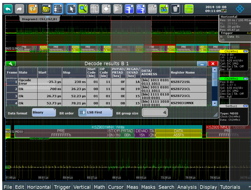
Figure 12-95: The same signal trace and decode results table as in the previous figure, but only with "DATA" in binary format
