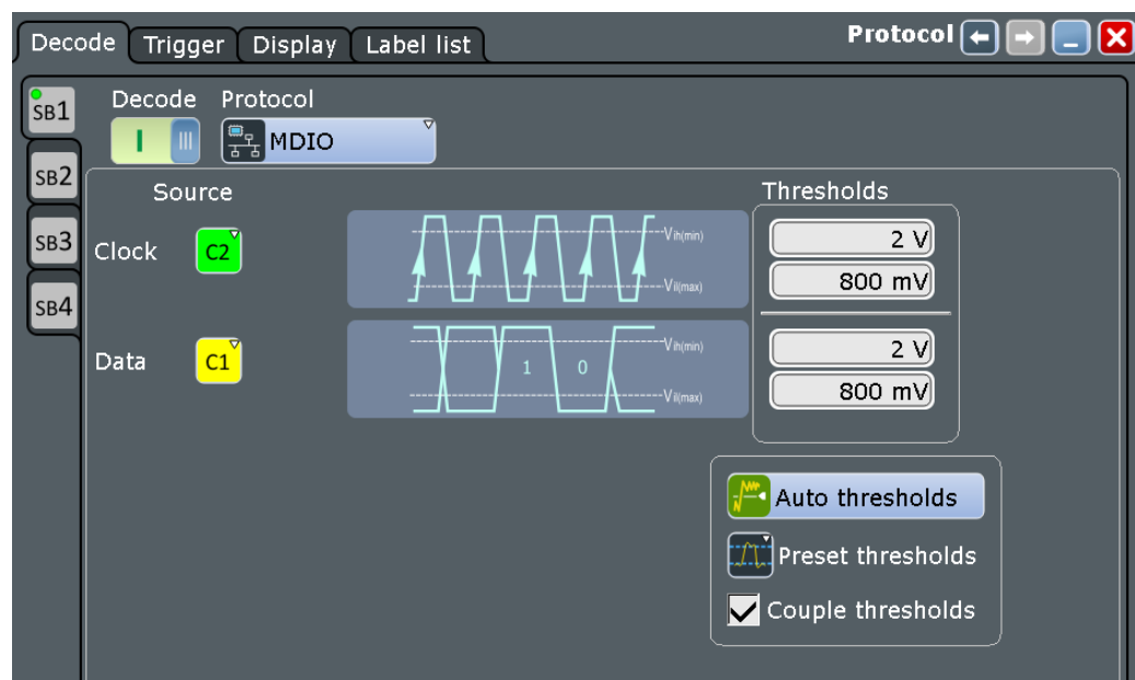
Figure 12-92: Serial bus MDIO protocol configuration dialog
