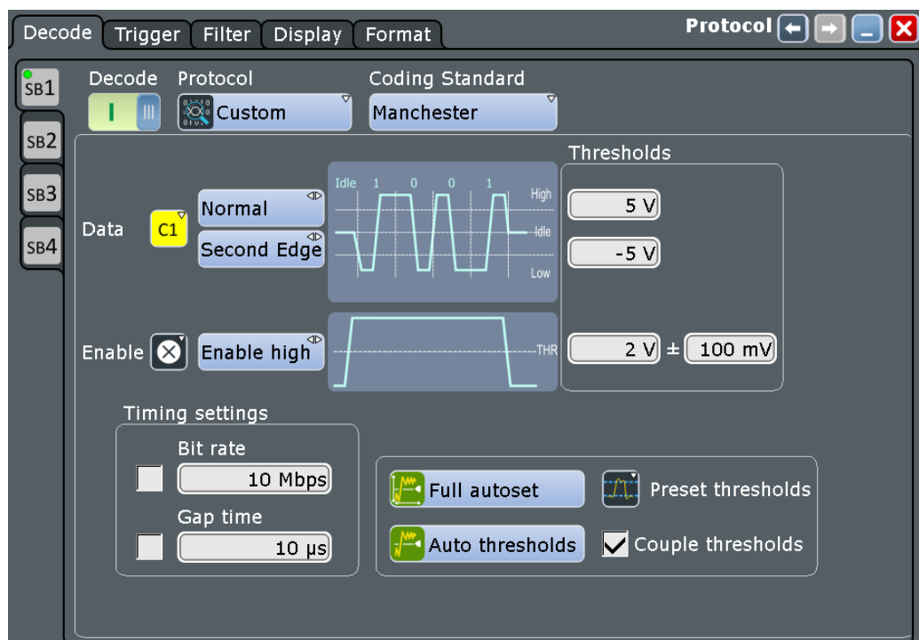
Figure 12-75: Coding standard selection in the serial bus protocol configuration dialog
