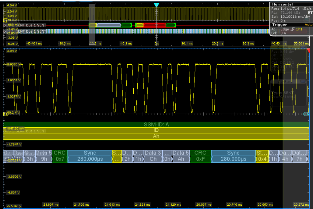
Figure 12-70: SENT decode results display
