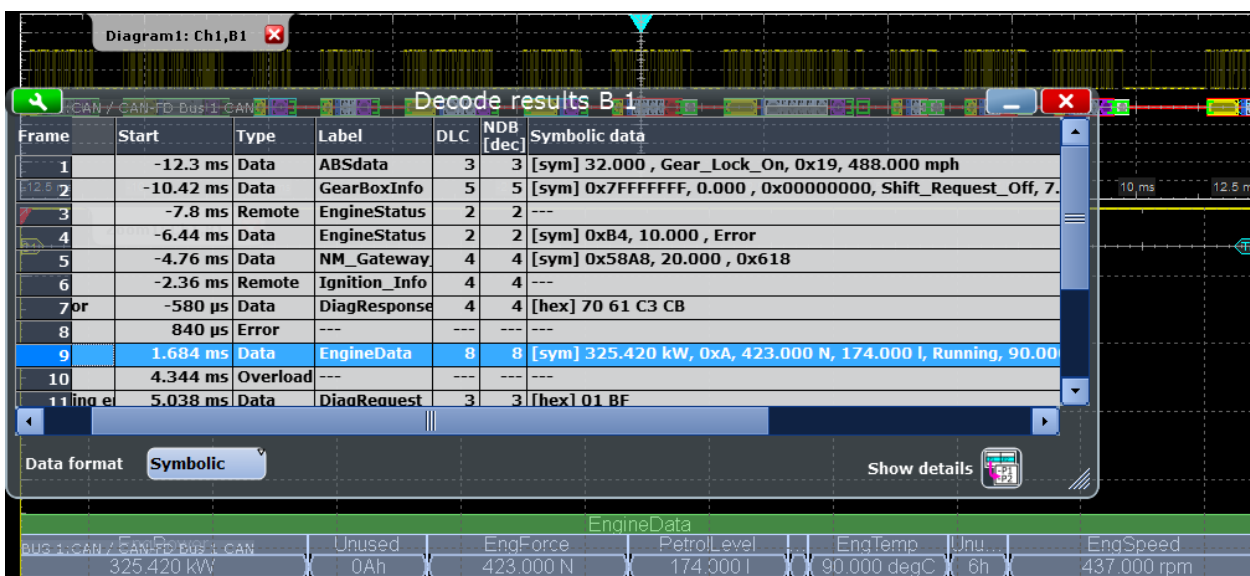
Figure 12-25: Decoded CAN signal with applied DBC file and "Symbolic" data in the result table
