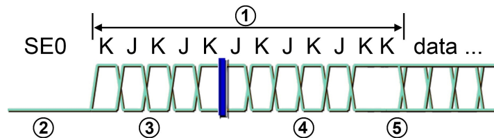
Figure 12-99: Start of a high-speed packet: after an SE0, the packet starts with a SYNC field (or SOP), followed by the data packet
