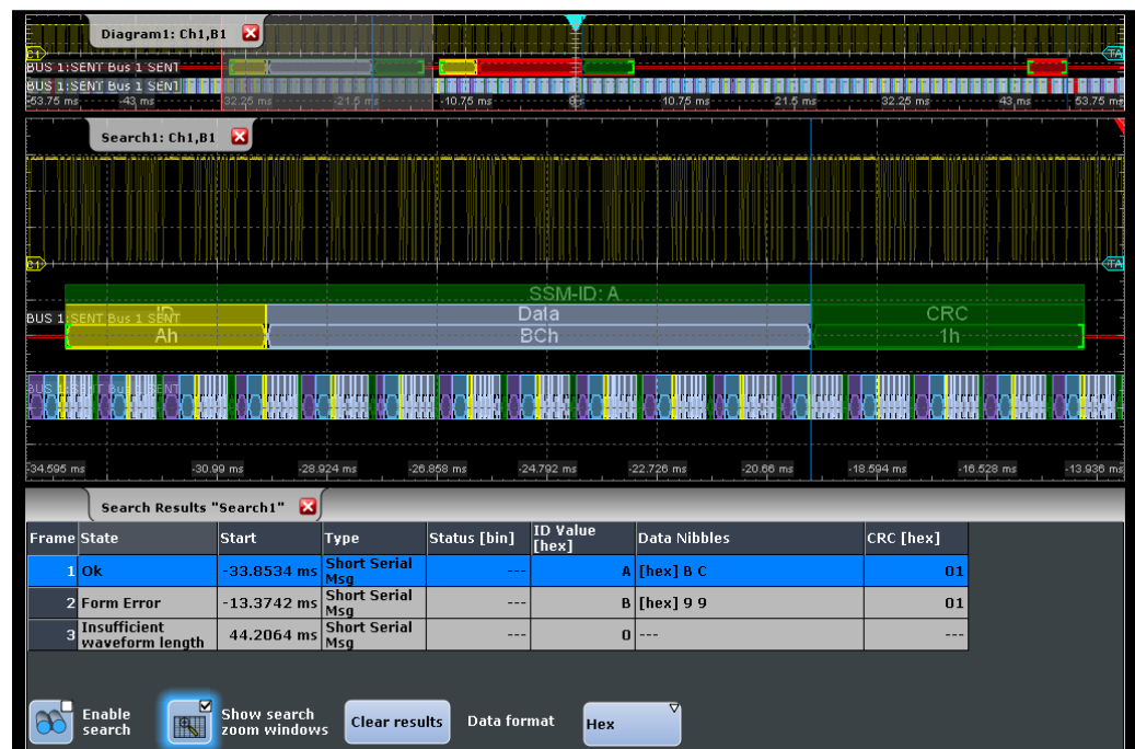
Figure 12-74: Search on the Status nibble in a SENT transmission signal
