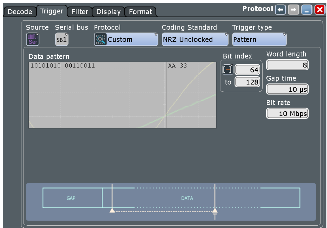
Figure 12-88: Custom serial bus: setting the pattern trigger, here for coding standard NRZ Unlocked
