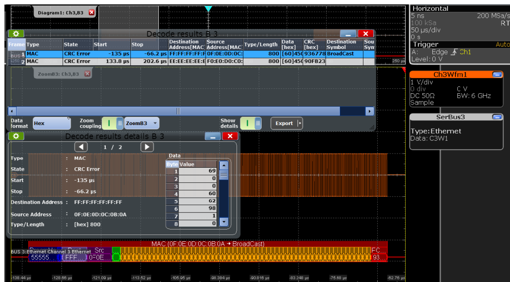
Figure 12-59: Ethernet 100BASE-TX: decoded and binary signal (zoomed view)
