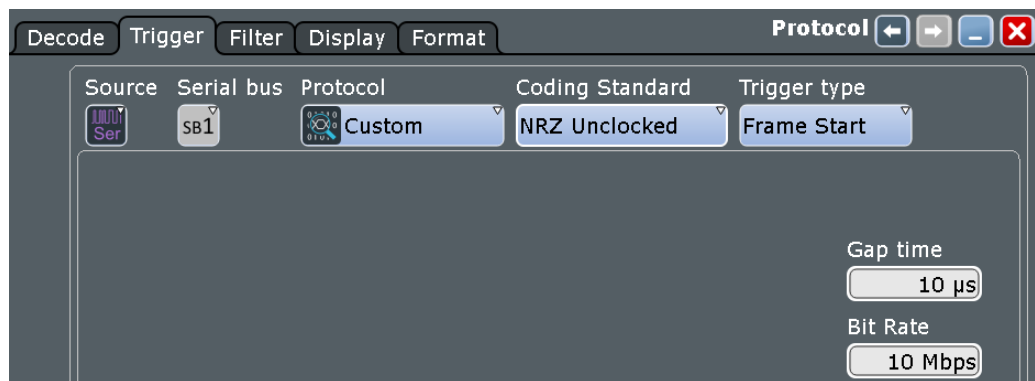
Figure 12-87: Custom serial bus: setting the trigger to frame start
