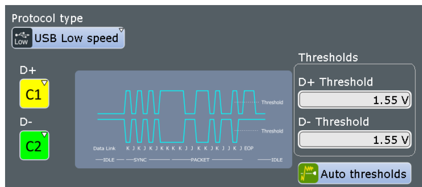
Figure 12-101: USB low speed protocol configuration
