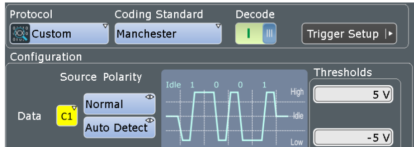
Figure 12-76: Custom serial bus coding configuration Manchester
