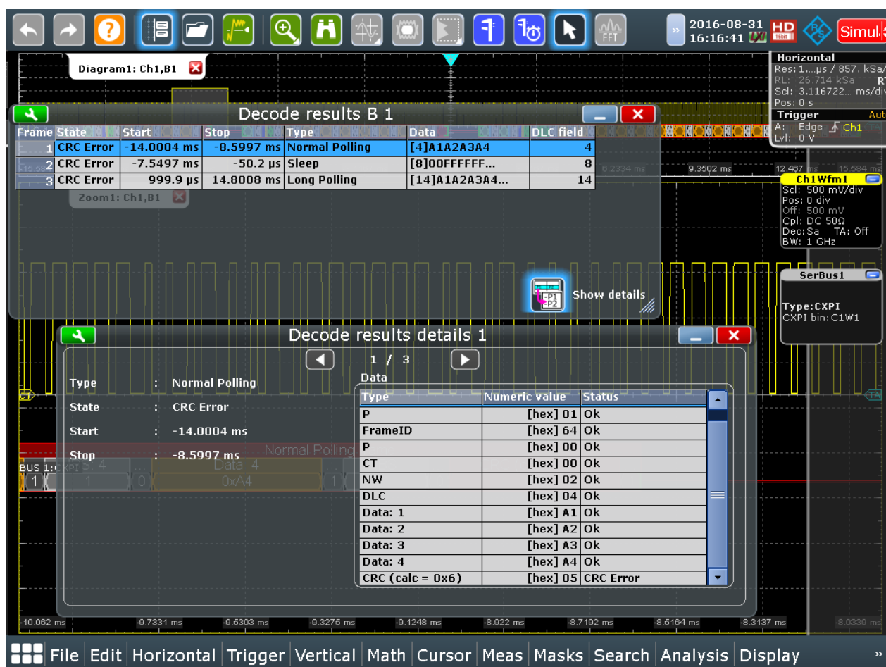
Figure 12-121: Decoded CXPI signal result tables, normal polling frame with CRC error
