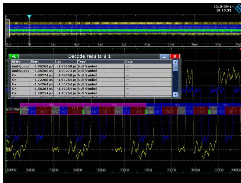
Figure 12-115: Decoded SpaceWire signal with ambiguous bits
