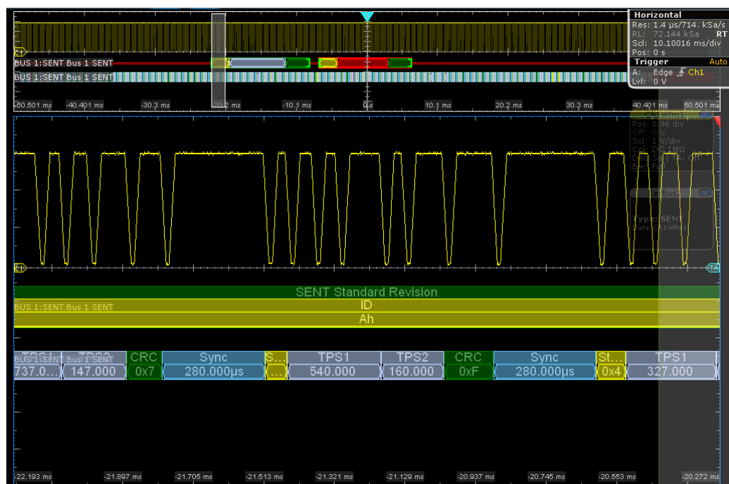
Figure 12-68: SENT decode results with label list translation
