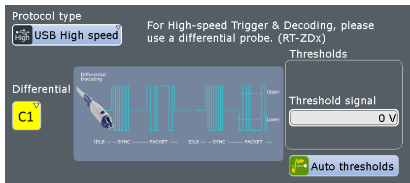
Figure 12-103: USB high-speed protocol configuration
