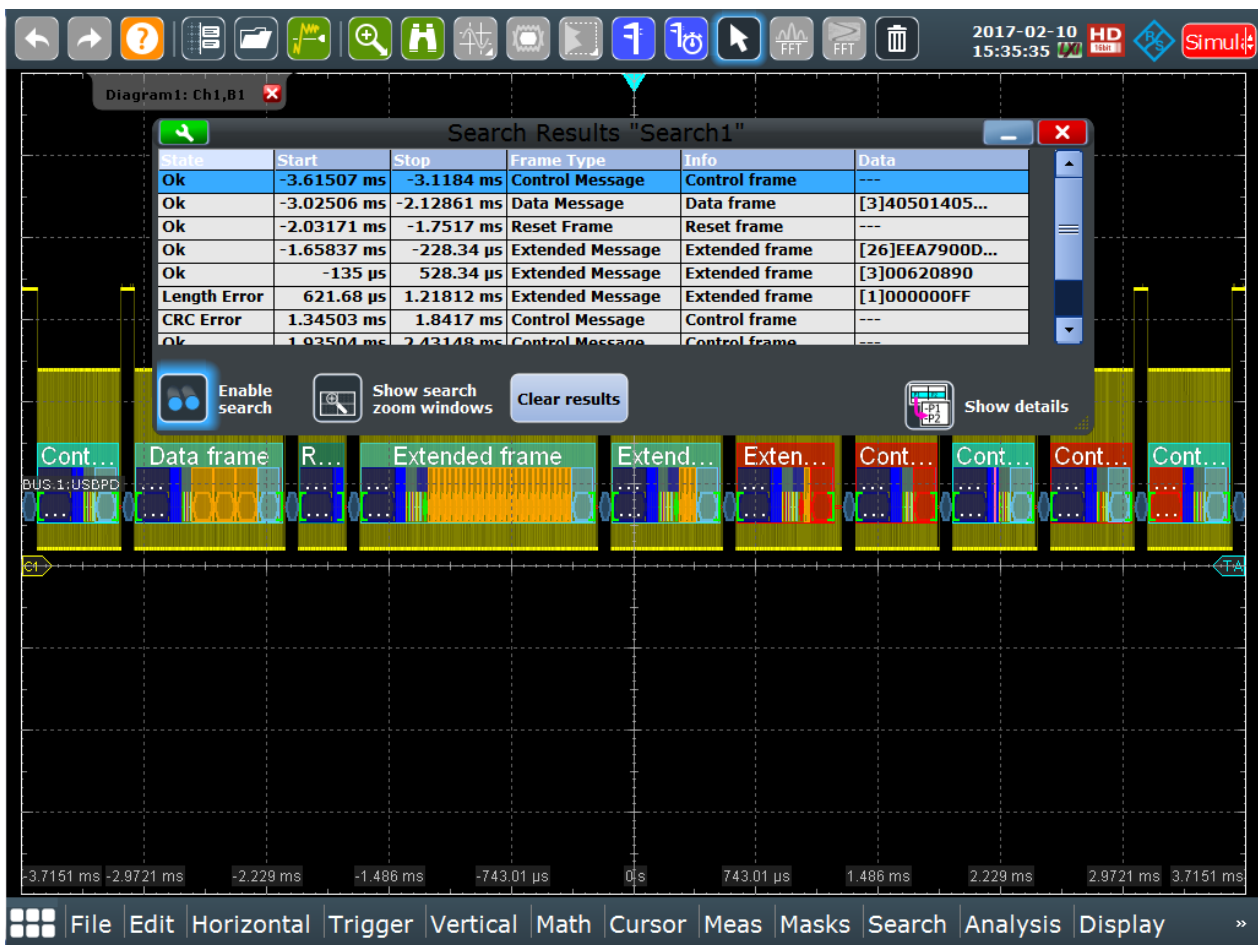
Figure 12-111: Search on USBPD frame
