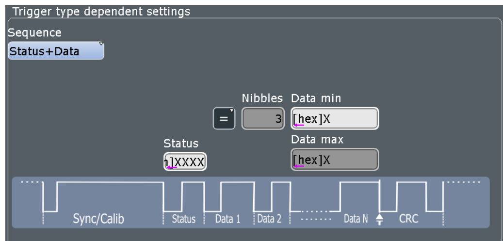
Figure 12-73: Search setting parameters of a transmission sequence
