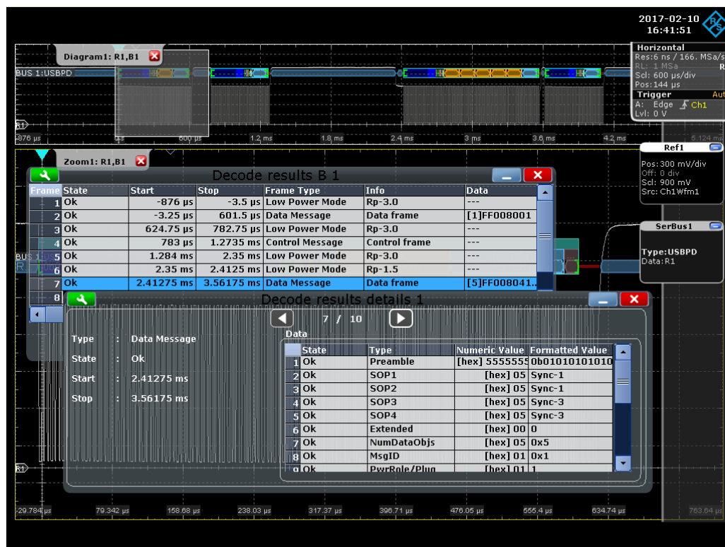
Figure 12-110: USBPD protocol: decoded and binary signal, and decode results
