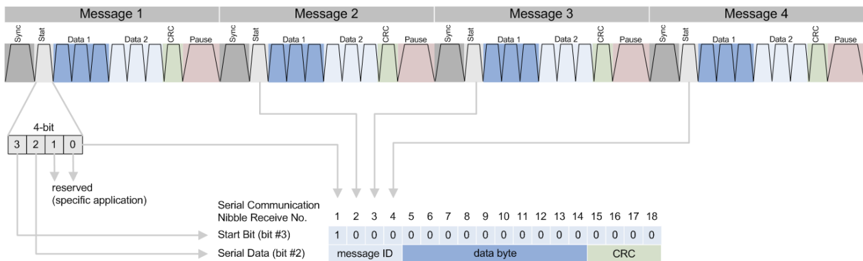
Figure 12-64: One serial message, composed of 16 SENT consecutive fast channel transmissions
