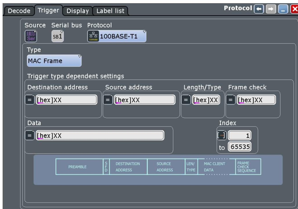
Figure 12-60: 100BASE-T1 trigger event settings dialog
