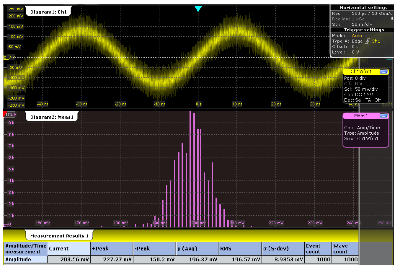
Figure 7-10: Statistical results and measurement histogram of an amplitude measurement
