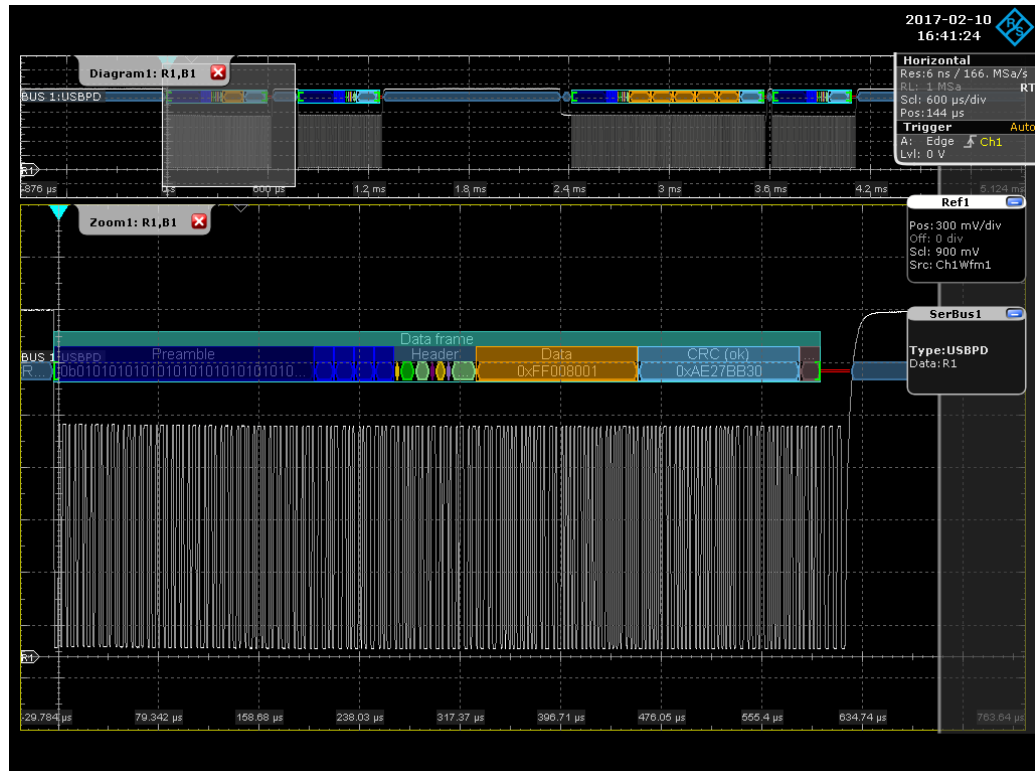
Figure 12-109: USBPD protocol: decoded and binary signal
