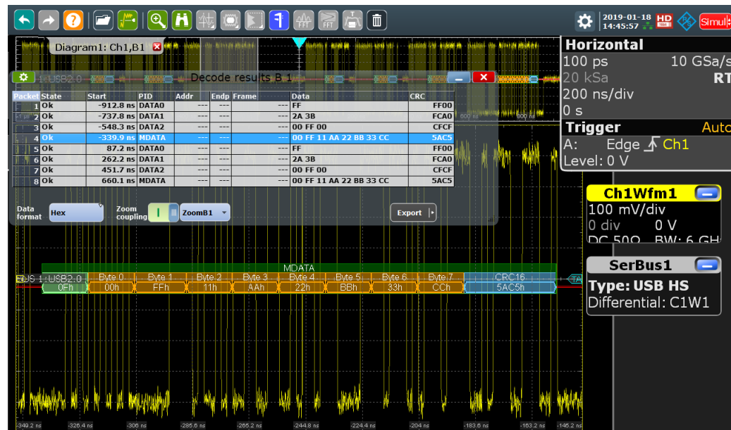
Figure 12-107: USB high-speed protocol: decoded and binary signal, and decode results
