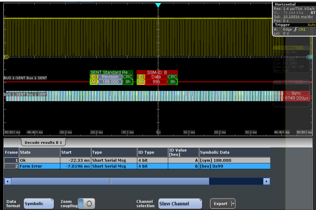
Figure 12-71: SENT decode results of a short serial message
