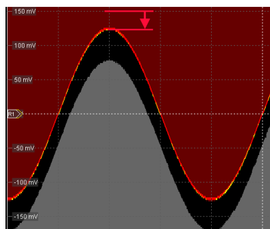
Figure 9-5: Waveform mask with vertical width = 0.5 div and vertical position = -0.5 div
