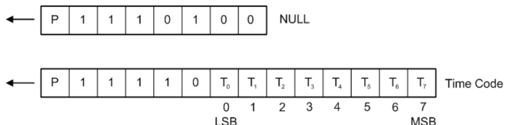
Figure 12-114: SpaceWire control codes
