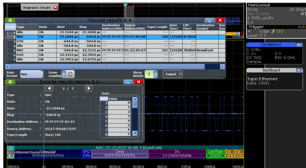
Figure 12-58: Ethernet 10BASE-T: decoded and binary signal, with decode results table and details
