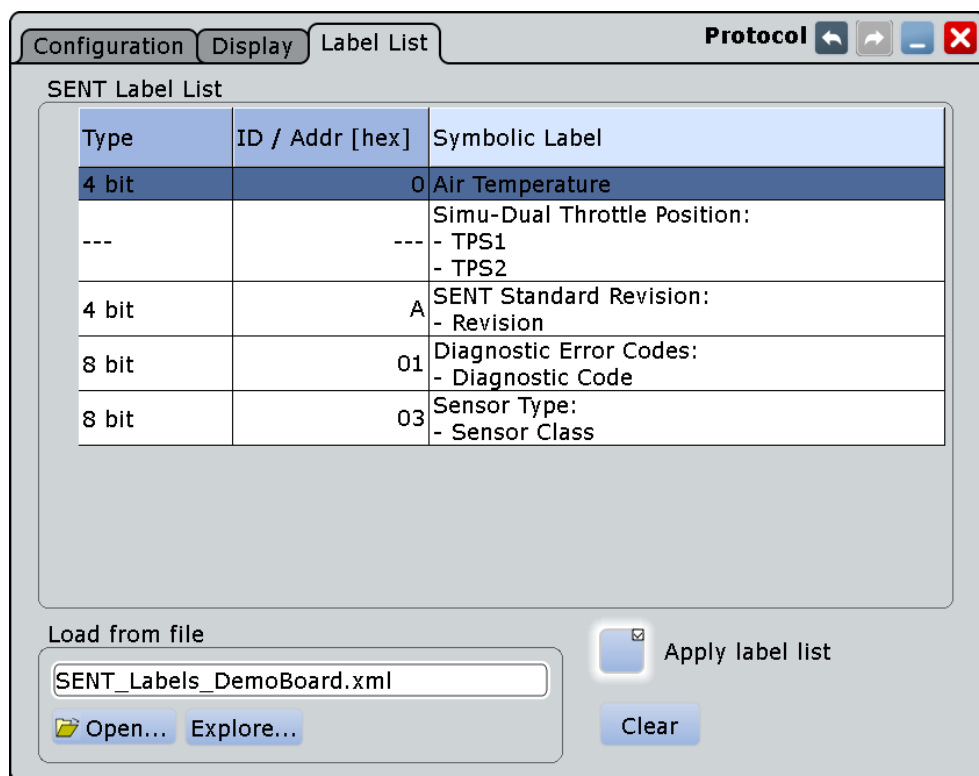
Figure 12-67: SENT label list
