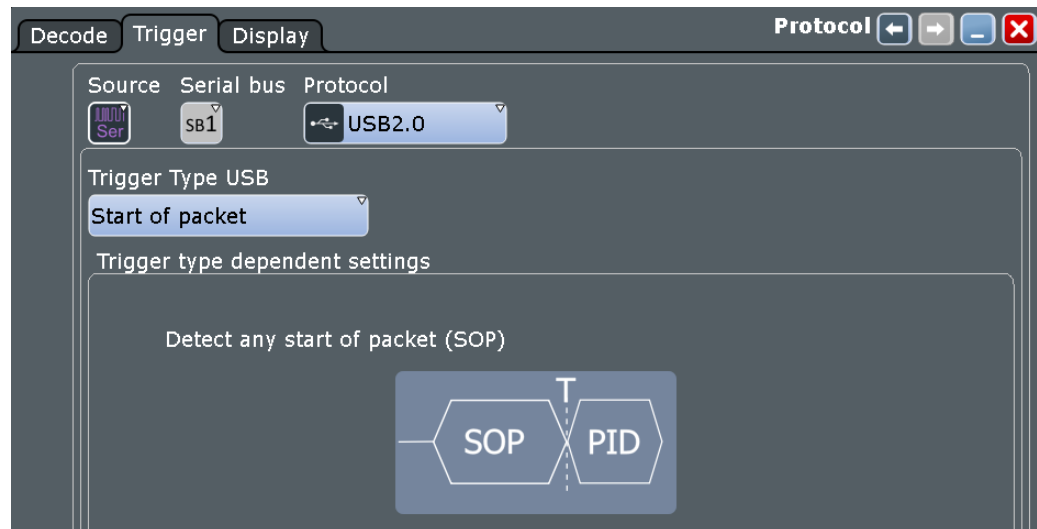
Figure 12-105: USB trigger event settings dialog
