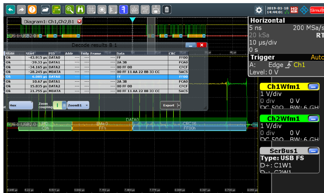
Figure 12-106: USB full speed protocol: decoded and binary signal, and decode results
