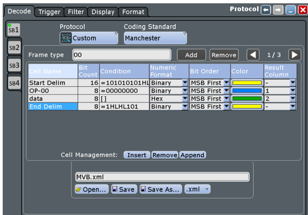
Figure 12-82: Example of a custom "ProfiBus Voltage" frame format description (frame 1 of 3)
