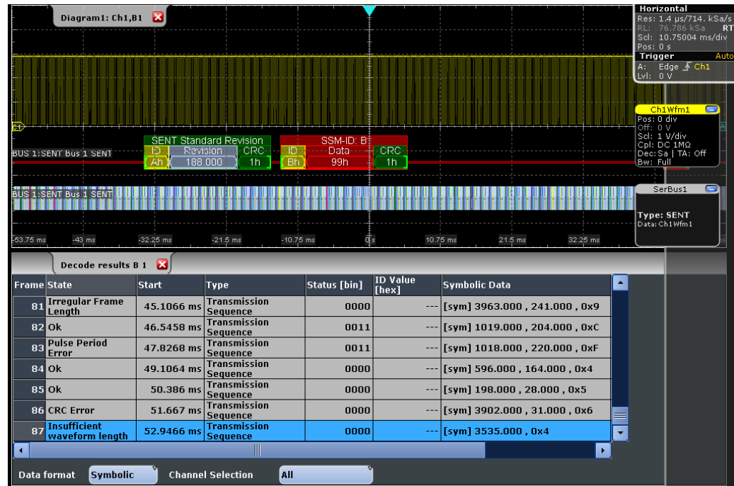
Figure 12-69: SENT label list translation
