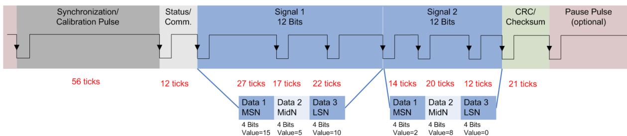
Figure 12-63: Example of a SENT transmission sequence
