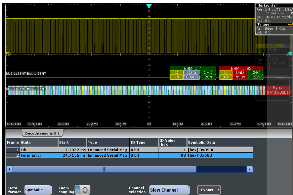
Figure 12-72: SENT decode results of an enhanced serial message
