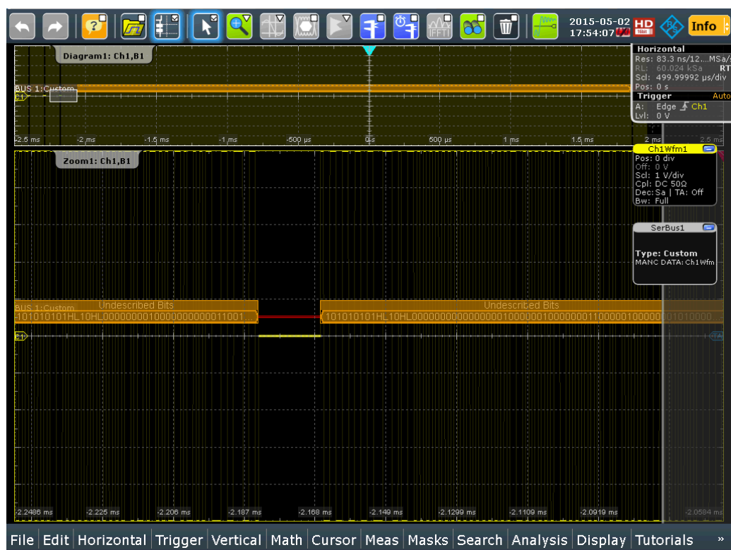
Figure 12-90: The function "Undescribed Bits" catches frames missed by the frame format descriptions
