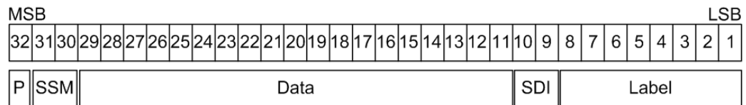
Figure 12-51: Structure of an ARINC 429 word
