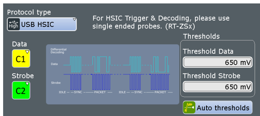
Figure 12-104: USB HSIC protocol configuration
