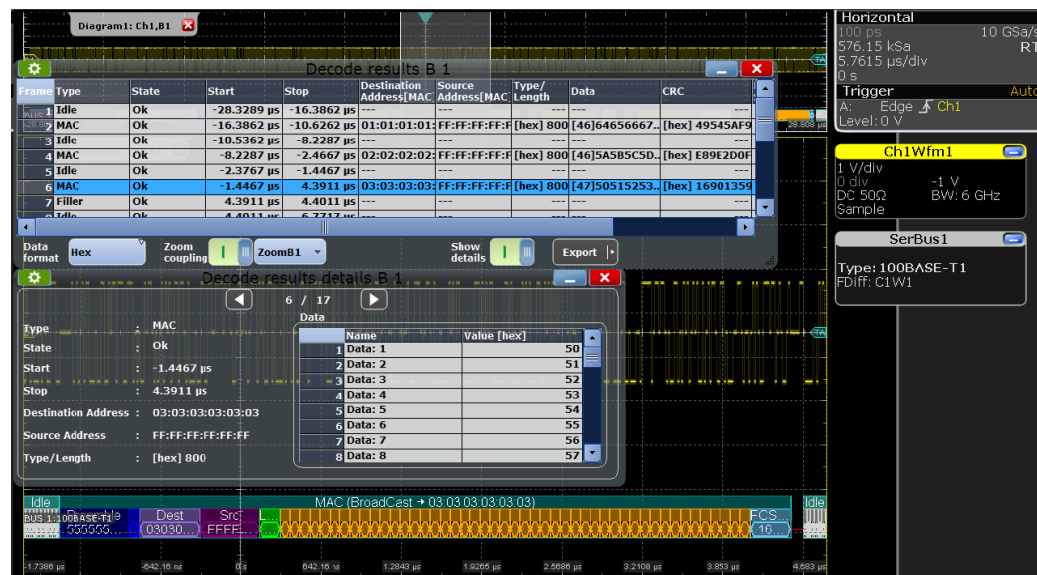
Figure 12-62: 100BASE-T1 decode results table and details
