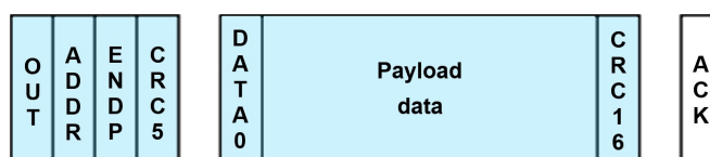
Figure 12-98: Example of a bulk OUT transfer. Blue: host speaks, white: device speaks
